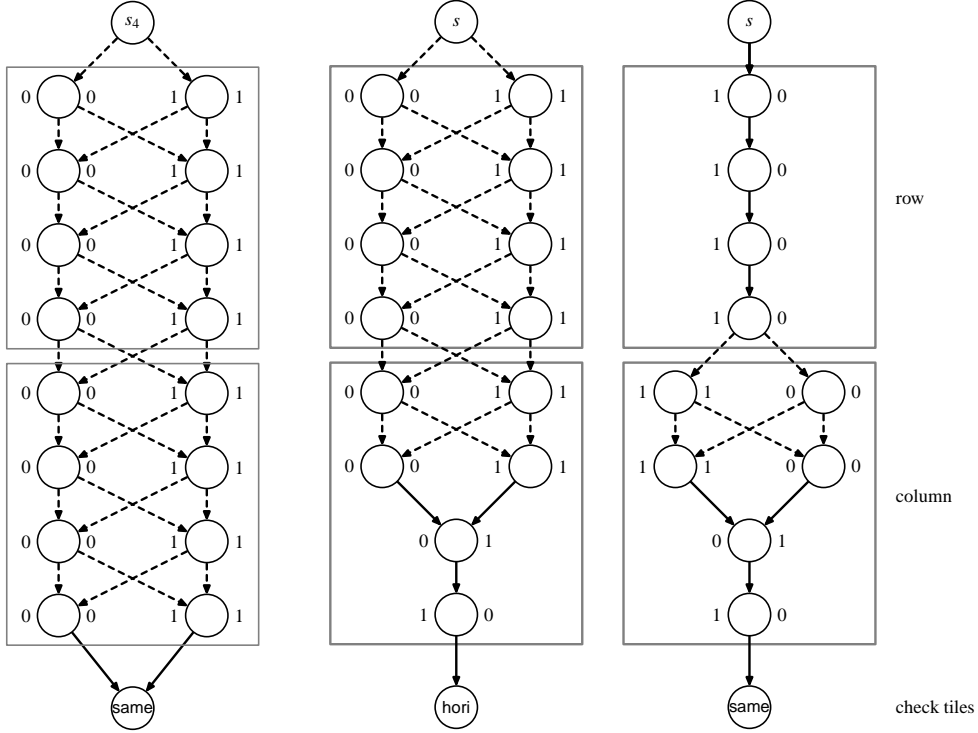
Figure 1: \mathcal{P}_4
