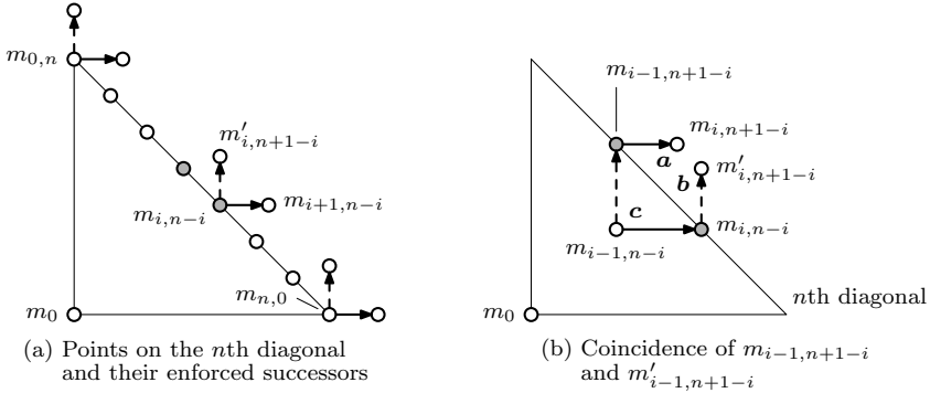
Fig. 2. The diagonal-wise construction of the grid
