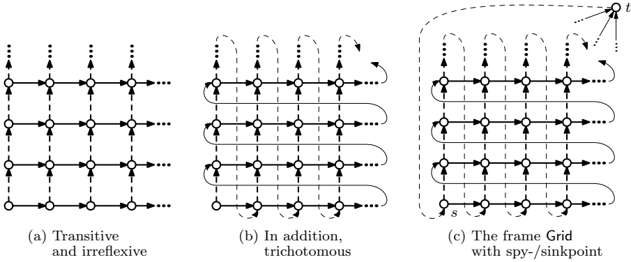
Fig. 1. Simulating the \mathbb{N} \times \mathbb{N} grid with two relations. The transitive closures are not drawn.
